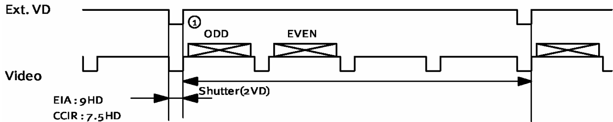
Fig. 24. Long time exposure. Frame accumulation.
