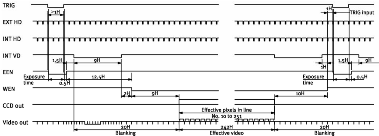
Fig. 20. Pulse width control EIA.
