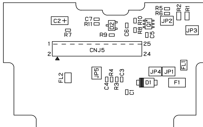
Fig. 31. PK8279 Rear Board of CV-A50/60
