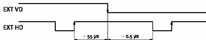
Fig. 16. Ext. HD and ext. VD phase conditions.
