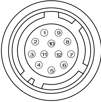
Fig. 2. 12-pin connector.
