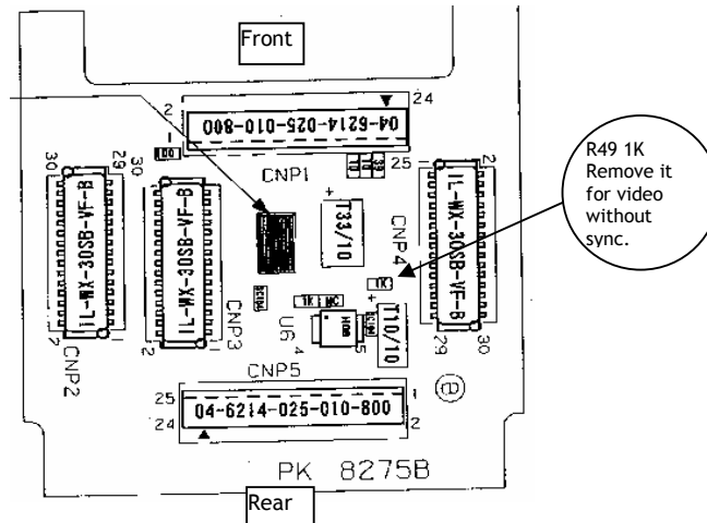
Fig. 33. PK8275B main board top side
