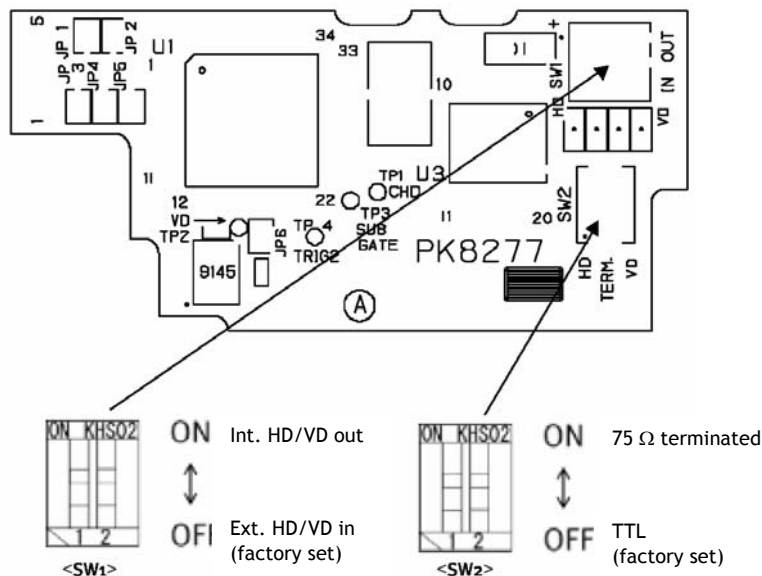
Fig. 29. HD/VD switch positions on PK8277 board.
