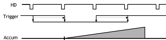
Fig. 8. PWC H synchronous accumulation.
