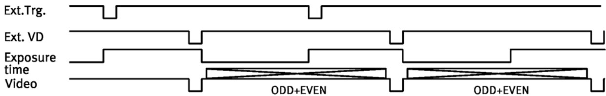
Fig. 25b. Start/stop mode. Interlaced with field accumulation.
