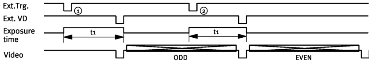
Fig. 25a. Start/stop mode. Interlaced with frame accumulation.
