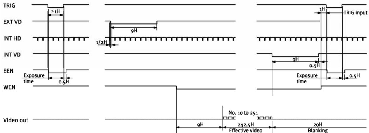
Fig. 22. Frame delay read out. EIA
