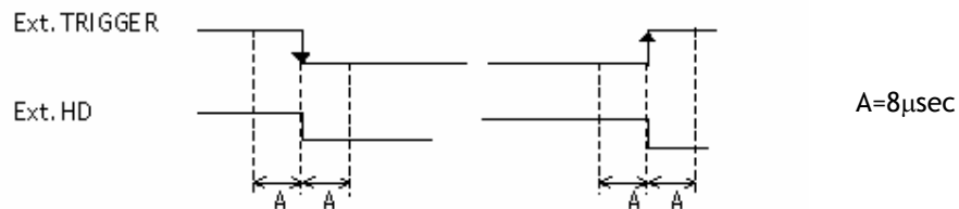
Fig. 14. Trigger/HD timing.
