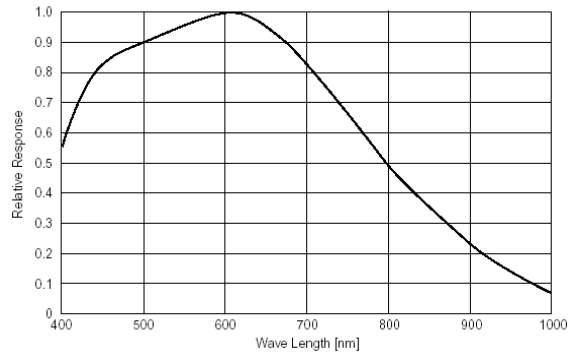
Fig. 30. Spectral sensitivity.
