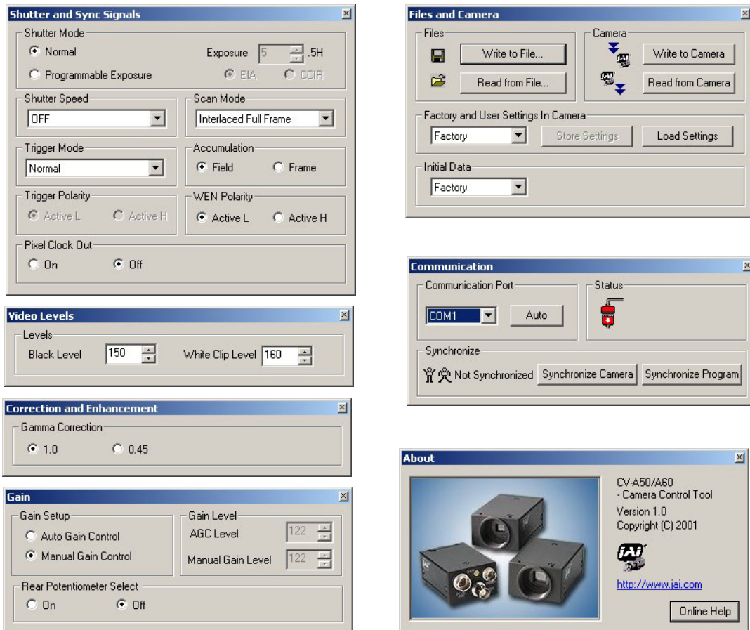
Fig. 28. Windows from Camera Tools.
