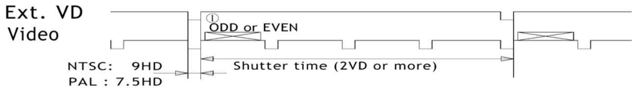
Fig. 27. Long time interlaced field integration
