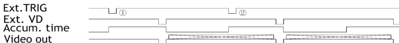
Fig. 23. Start stop interlaced field integration
