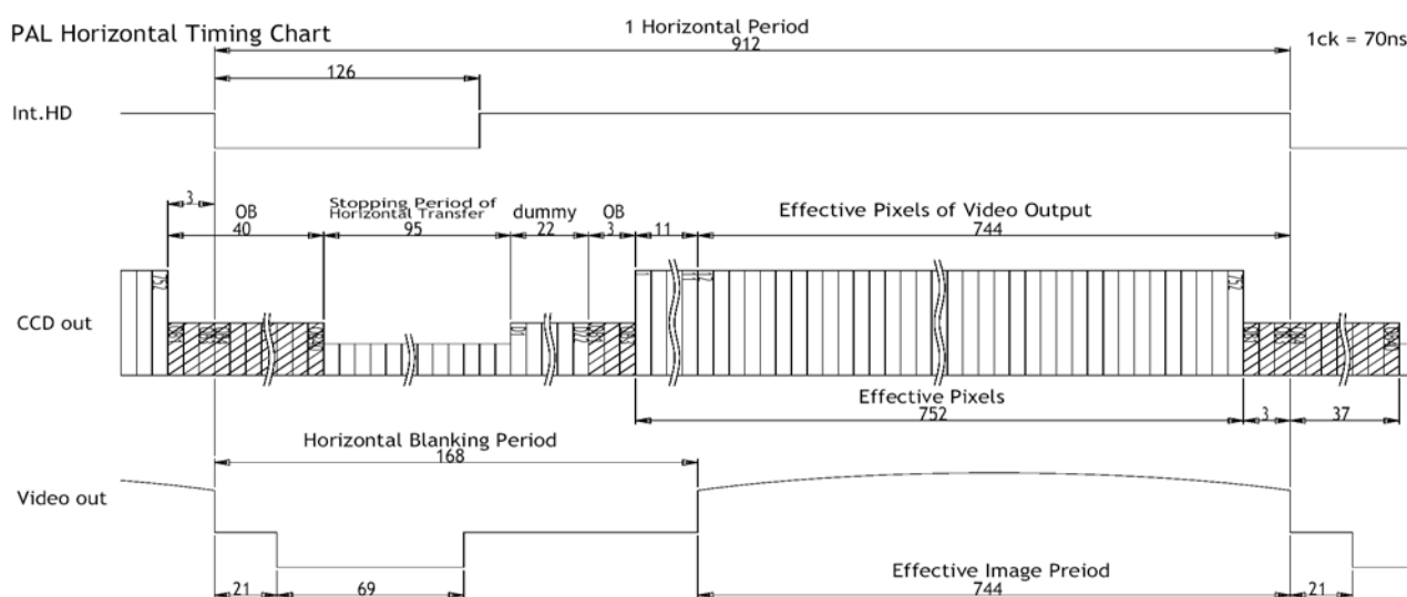
Fig. 13. PAL horizontal timing
